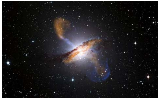
Centaurus A, Credit: NASA http://www.nasa.gov/images/content/312037main_cena_full.jpg
